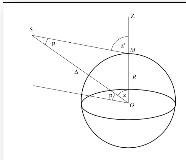
FIGURE 1. – LA PARALLAXE HORIZONTALE.
